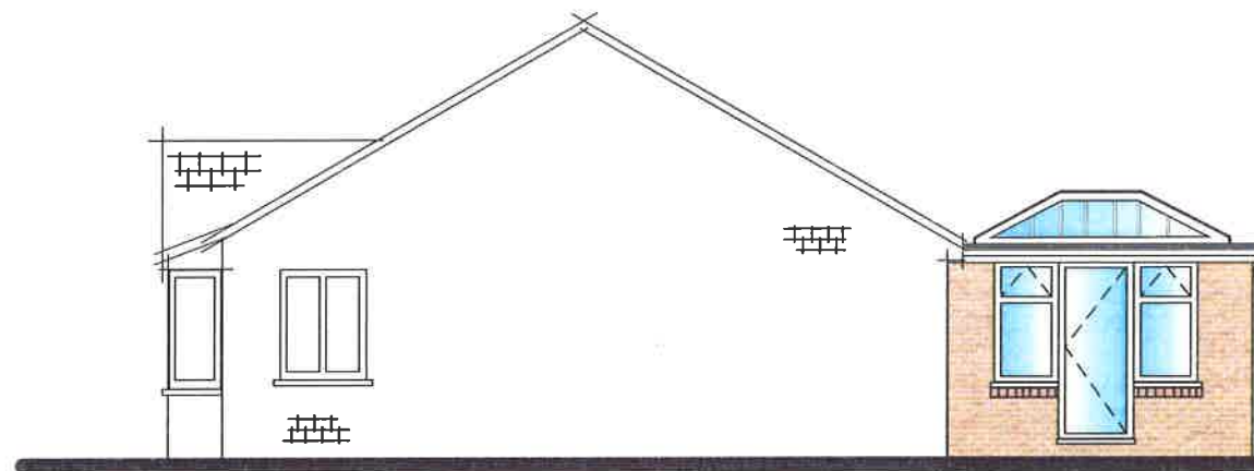
PROPOSED SIDE ELEVATION (EAST)
